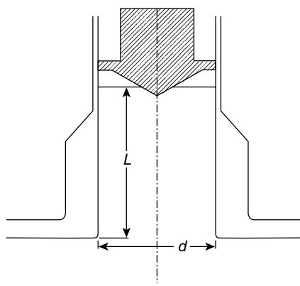
FIGURE 10.3 Safety valve arrangement
