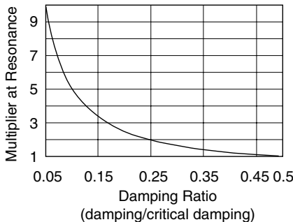
FIGURE 10.2 Multiplier effect of damping ratio
