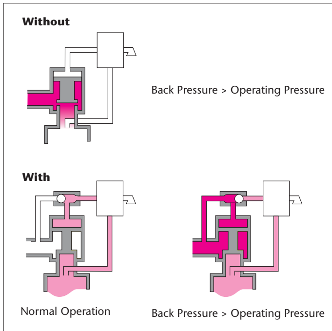
Back Flow Preventer
