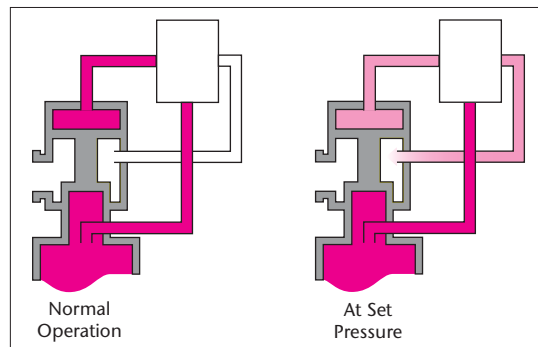
Pilot Vented to Body Bowl / Outlet Flange
