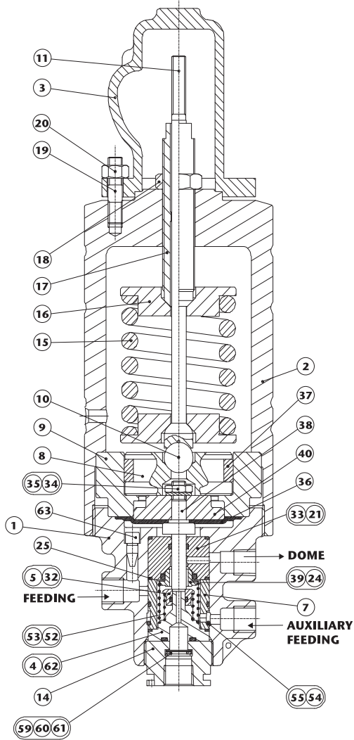
Diaphragm design for pressures upto 36 barg (522 psig)
