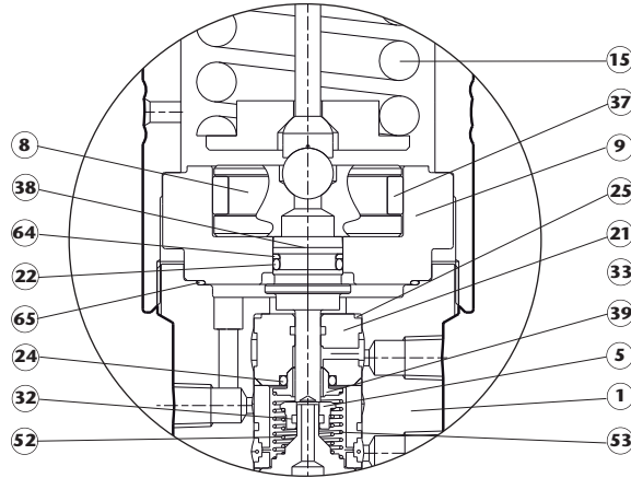
Piston design for pressures over 36 barg (522 psig)
