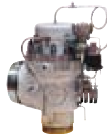
86 Series Hot service - Full nozzle API spring loaded SRV dimensions Set pressure : up to 180 barg Temp : up to 550°C
