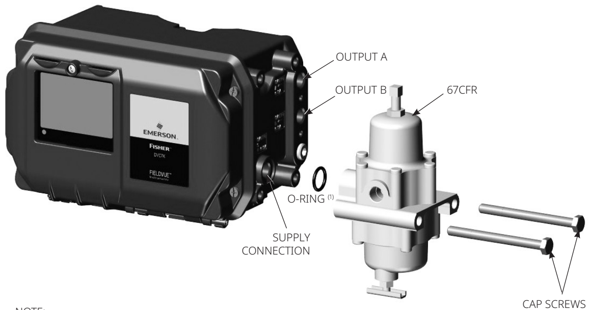
Figure 15. Integral Mounting of a Fisher 67CFR Regulator on a FIELDVUE DVC7K Digital Valve Controller
